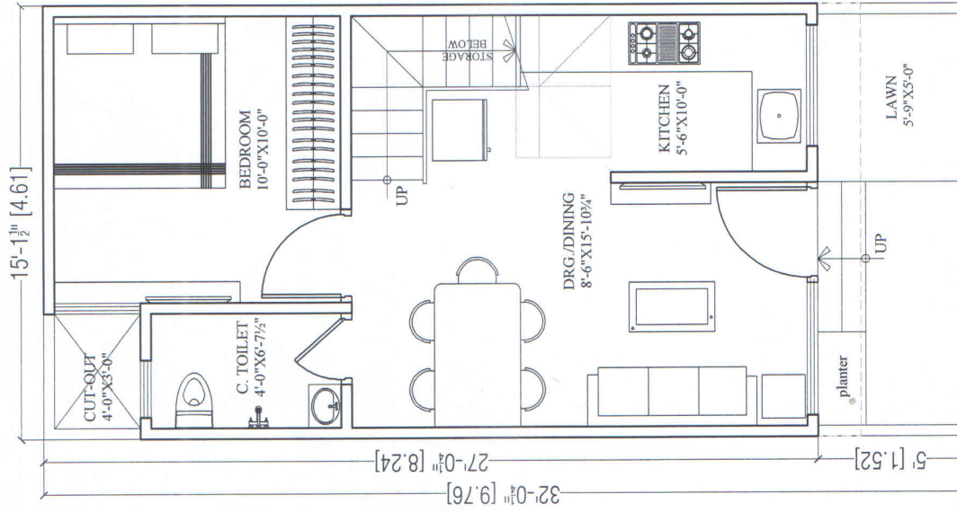
GROUND FLOOR PLAN CARPET AREA = 315.75 SQ. FT. BUILT-UP AREA = 416.68 SQ. FT.
